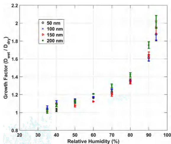
Fig. 5. Increasing RH growth factor variations different dry sizes of CsOH particle
