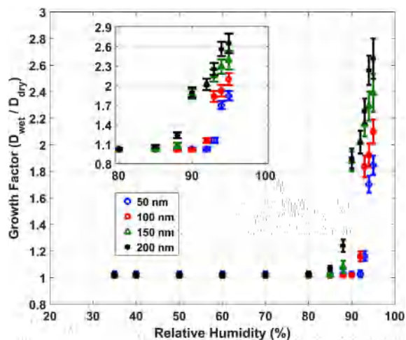
Fig. 3. Increasing RH growth factor variations for different dry sizes of CsI particle
