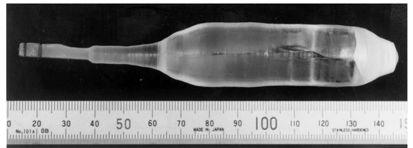
Fig. 7. As-grown Ce-doped LiCaAlF 6 single crystal with white substance at the bottom of the crystal and a large crack parallel to the growth axis.
