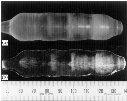
Fig. 5. Ce-doped LiCaAlF 6 crystal with inclusions: (a) as-grown crystal and (b) wafer cut parallel to the growth axis.
