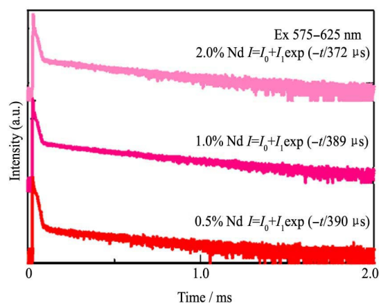
Fig. 4 PL decay time profiles of the Nd:SrAl 2 O 4 crystals
