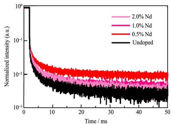
Fig. 8 Afterglow curves of the Nd:SrAl 2 O 4 crystals after the X-ray irradiation was cut off
