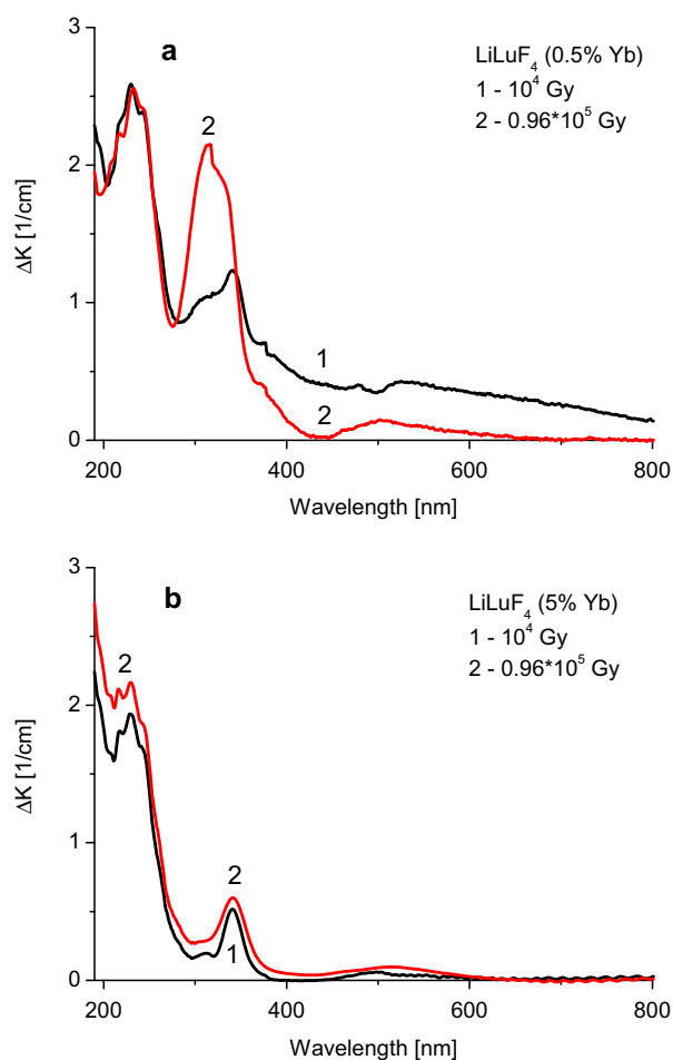
Fig. 2. Induced absorption of: (a) 0.5% Yb-doped \text{LiLuF}_4 and (b) 5% Yb-doped \text{LiLuF}_4 .
