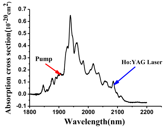
Fig. 2. Absorption cross section of Ho:SSO crystal.
