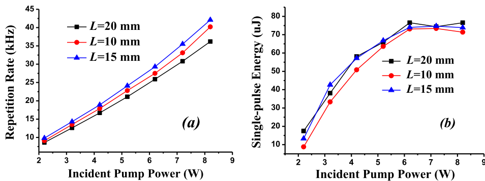
Fig. 5. (a) Repetition frequency; (b) Pulse energy as a function of incident pump power.
