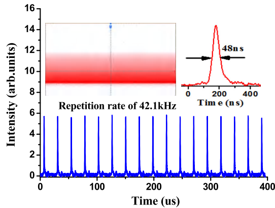
Fig. 7. Pulse trains of the PQS Ho:YAG laser. Inset, profile of the pulse.
