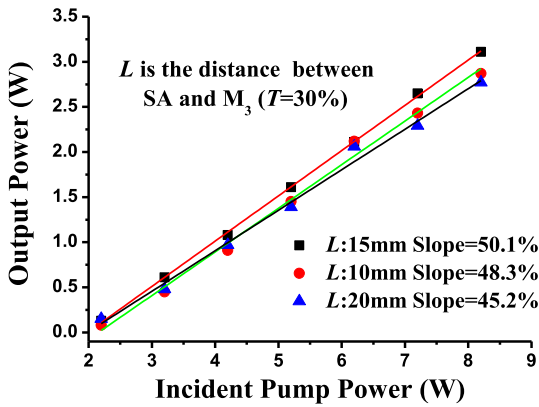
Fig. 4. Output characteristics curve of the PQS Ho:YAG laser.
