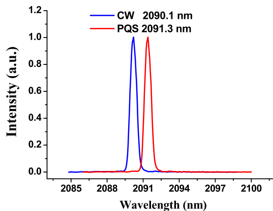
Fig. 8. Output spectra of the CW and PQS Ho:YAG laser.
