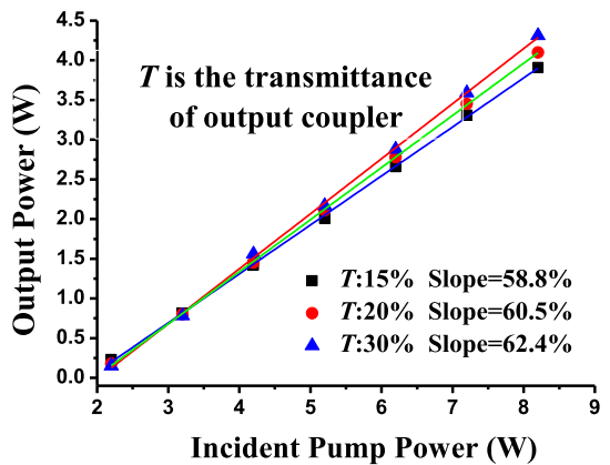
Fig. 3. Output characteristics curve of the free-running Ho:YAG laser.
