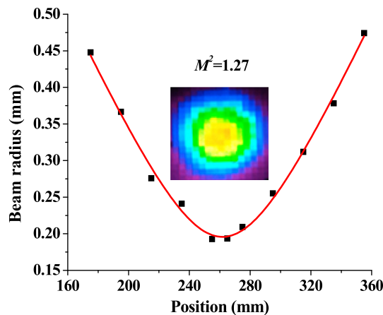
Fig. 9. The beam radius of the PQS Ho:YAG laser. Inset: typical 2D beam profiles.
