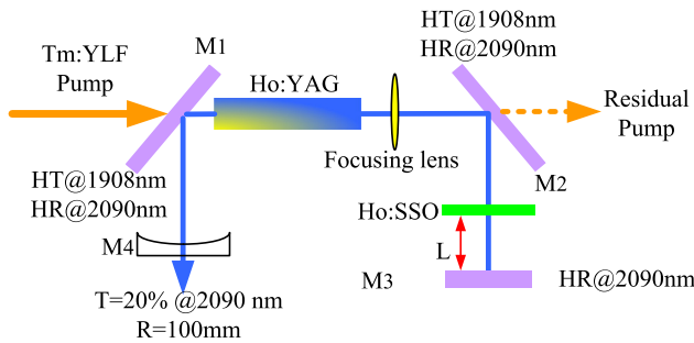
Fig. 1. Schematic diagram for the PQS Ho:SSO laser.
