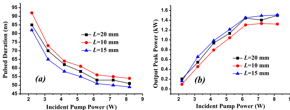
Fig. 6. (a) Pulsed duration; (b) Peak power as a function of incident pump power.
